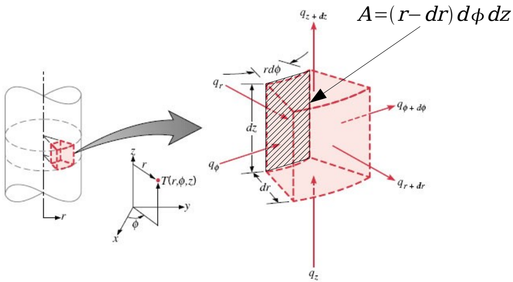
FIGURE 2.12 Differential control volume, dr \cdot r d\phi \cdot dz , for conduction analysis in cylindrical coordinates (r, \phi, z) .
