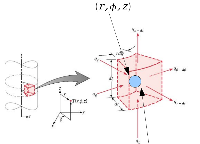
FIGURE 2.12 Differential control volume, dr \cdot r d\phi \cdot dz , for conduction analysis in cylindrical coordinates (r, \phi, z) .
