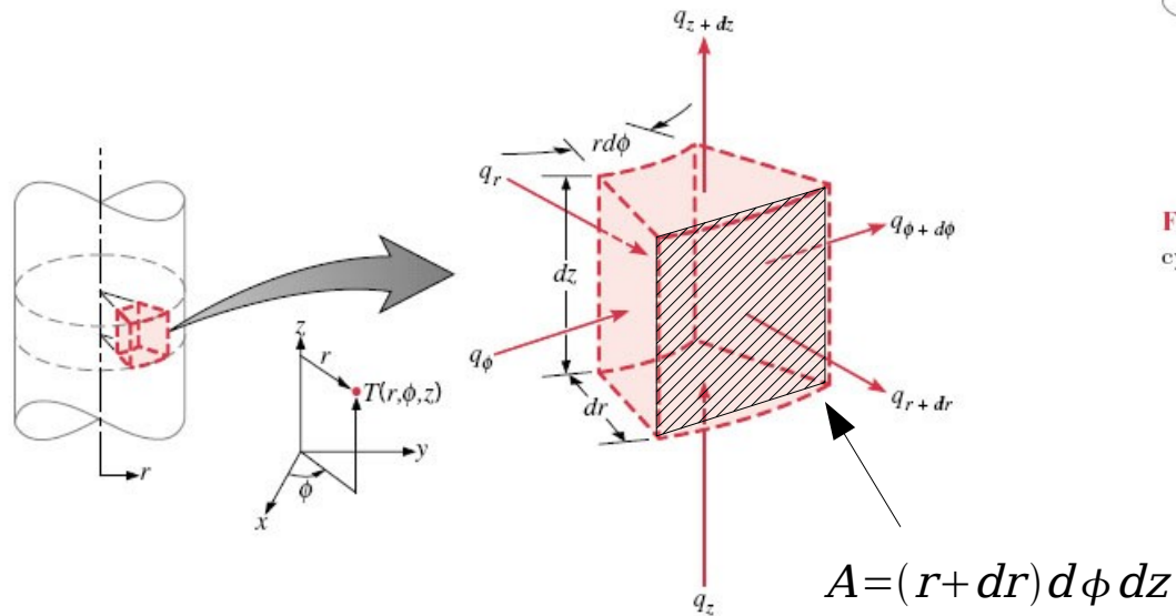
FIGURE 2.12 Differential control volume, dr \cdot r d\phi \cdot dz , for conduction analysis in cylindrical coordinates (r, \phi, z) .
